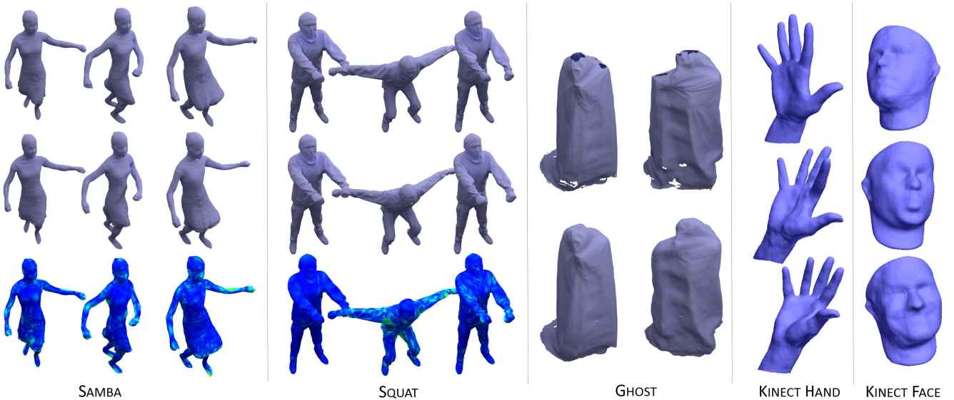
Figure 11: Comparison of our real-time reconstruction (top row) with offline reconstructions [Li et al. 2009] while only using depth data (i.e., no color term).
