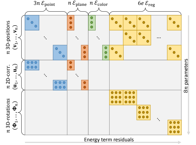
Figure 5: Block structure of the (\mathbf{V}, \mathbf{U}, \Phi) Jacobian (transposed). The Jacobian is never stored explicitly; instead the products J\mathbf{h} and J^\top \mathbf{h} are computed on demand on the GPU.
